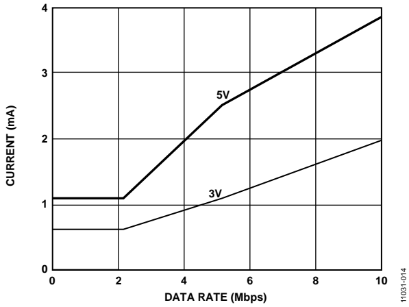
Figure 14. Typical ADuM4401W V_{DD2} Supply Current vs. Data Rate for 5V and 3V Operation
