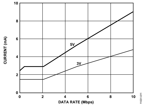
Figure 11. Typical ADuM4400W V_{DD1} Supply Current vs. Data Rate for 5V and 3V Operation
