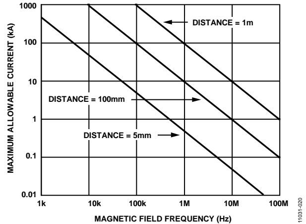
Figure 20. Maximum Allowable Current for Various Current-to-ADuM440xW Spacings
