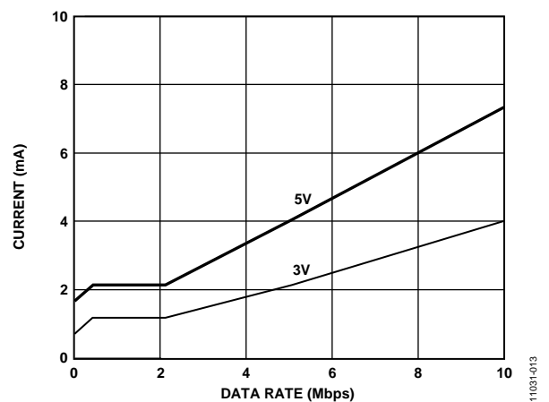
Figure 13. Typical ADuM4401W V_{DD1} Supply Current vs. Data Rate for 5V and 3V Operation
