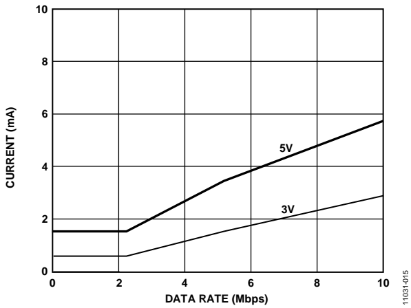
Figure 15. Typical ADuM4402W V_{DD1} or V_{DD2} Supply Current vs. Data Rate for 5V and 3V Operation
