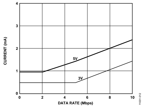
Figure 12. Typical ADuM4400W V_{DD2} Supply Current vs. Data Rate for 5V and 3V Operation
